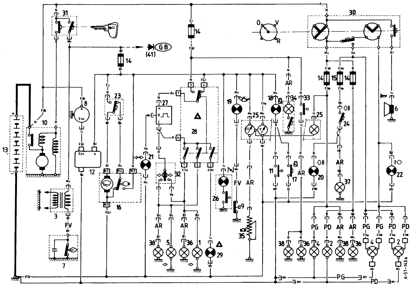
Fig. 4-5 1987 Standard 2CV Electrical Wiring Diagram
