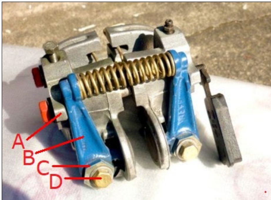
Fig. 2-1 Brake Caliper
